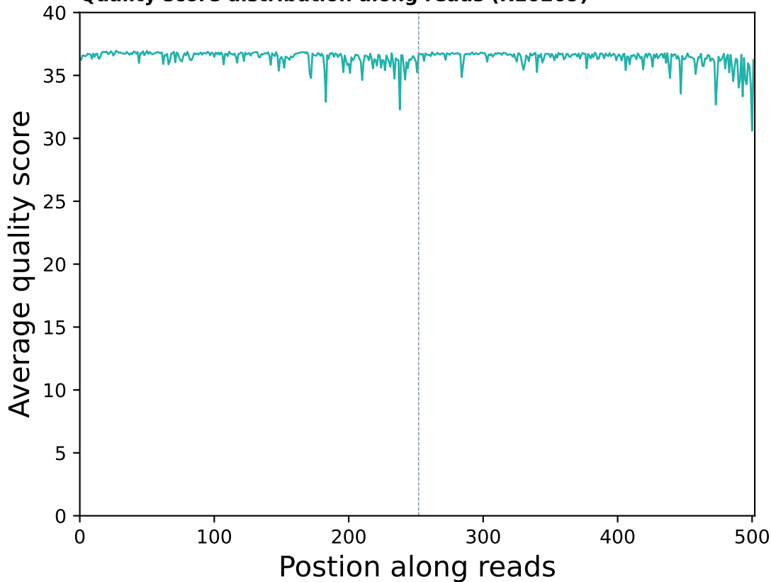
Quality score distribution along reads (R10209)
